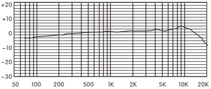
Frequency Response
