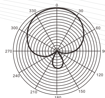
Polar Pattern
