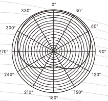
Polar Pattern
