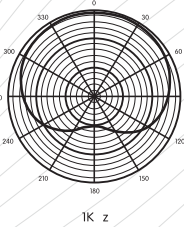
Polar Patterns
