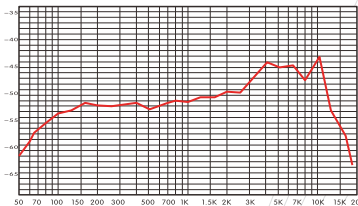
Spectrum Graph
